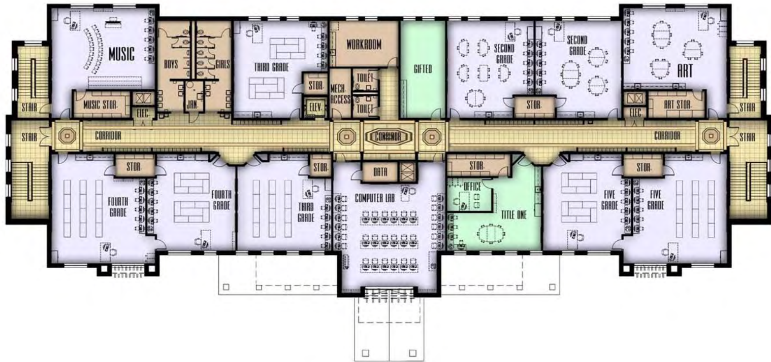
OVERALL SECOND FLOOR PLAN
